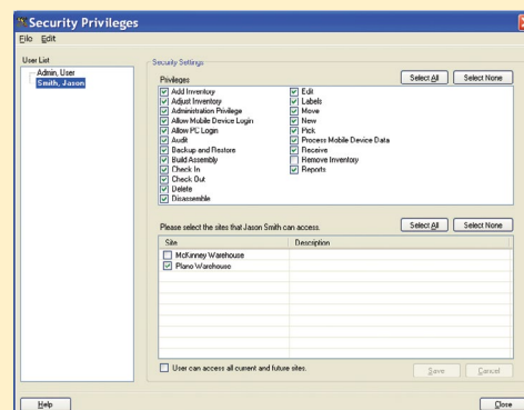
► Feature-based security
